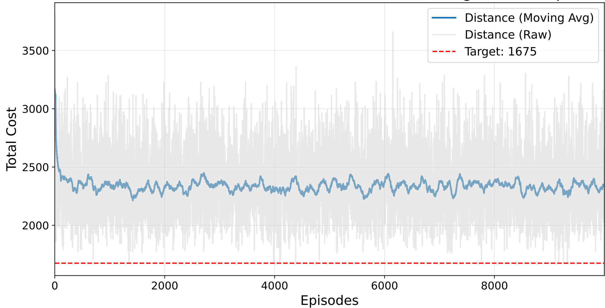
Final HYPERBAND TPE Masked AutoRL-SOP Training - ESC12.sop
